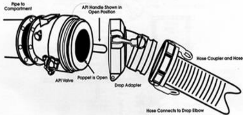
ILLUSTRATION F: API VALVE CONNECTION TO DROP HOSE AT SERVICE STATION
