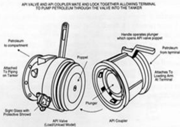
ILLUSTRATION E: API VALVE AND API COUPLER MATE AT TERMINAL
